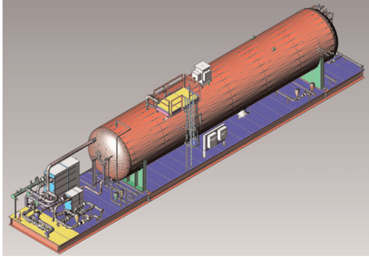
Electrostatic Heater Treater
